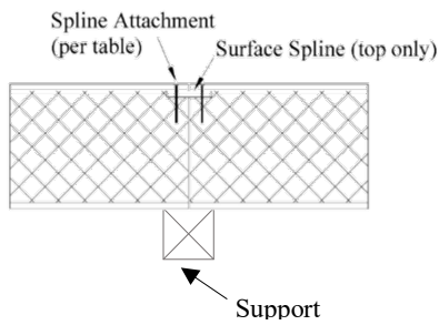
FIGURE 3A—INTERIOR SUPPORT SPLINE
