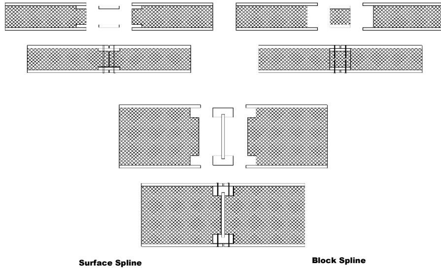
FIGURE 1—SIP SPLINE TYPES
