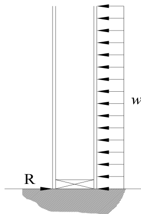
FIGURE 2—ZERO BEARING SUPPORT
