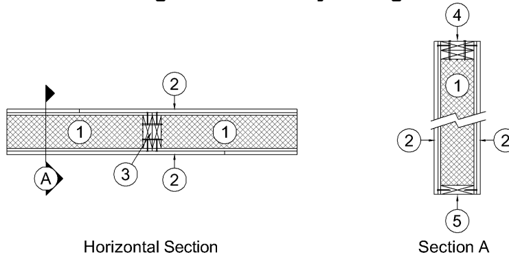
FIGURE 6—ASSEMBLY DRAWING FOR FIRE RESISTANCE SECTION 4.2.11.2
