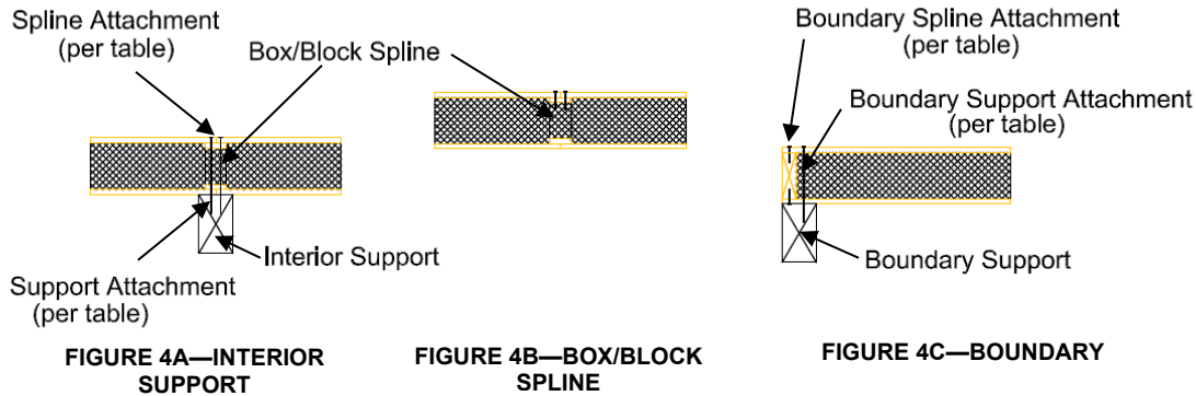
FIGURE 4—DIAPHRAGM CONNECTION TYPES
