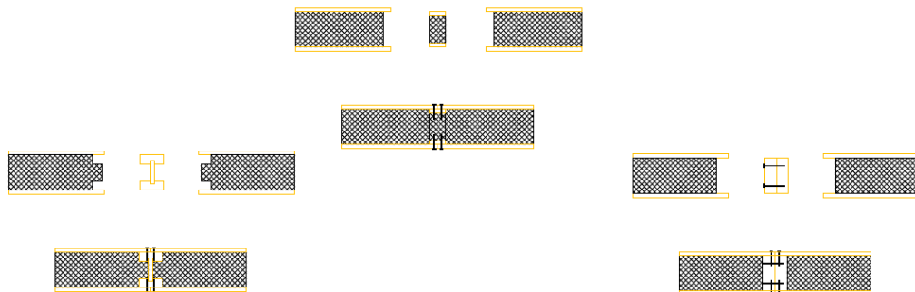
FIGURE 1—PREMIER SIP SPLINE TYPES
