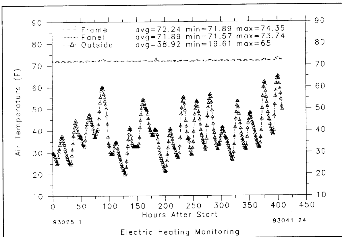
Figure 6a Hourly averages of inside temperature for both houses, and outside temperature, during the electric heating monitoring period
