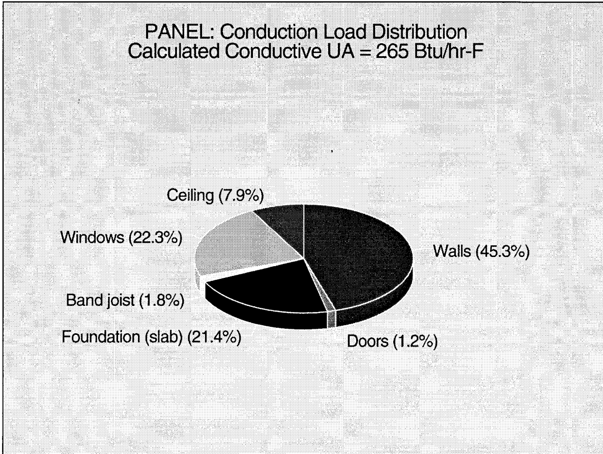
Figure 3b Conduction heating load distribution and calculated conductive UA for the SSIC panel house
