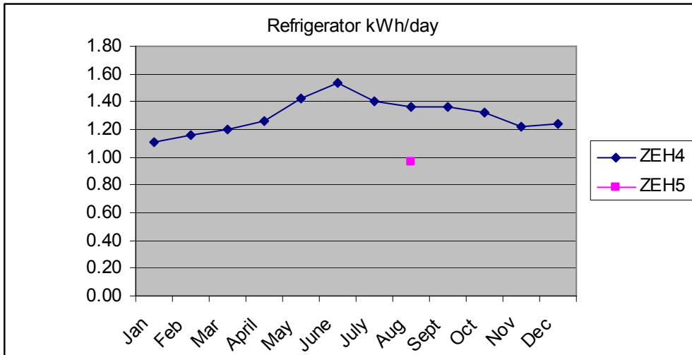
Figure 49. Daily energy demand for an 18-ft 3 Energy Star refrigerator, for all months in 2006 in ZEH4, which was occupied by three persons, and in August 2007 only in ZEH5, which was used only as an office.
