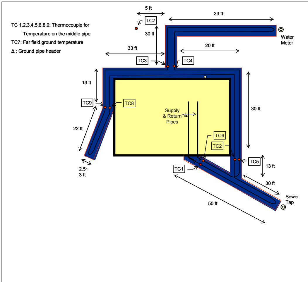
Figure 33. Locations and lengths along trenches where ground heat exchanger pipe was installed for ZEH5.
